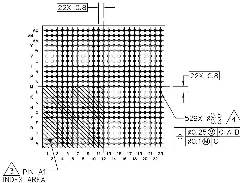
BOTTOM VIEW
