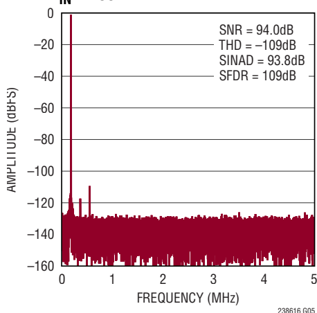
32k Point FFT f_{\text{SAMPL}} = 10\text{Mps} , f_{\text{IN}} = 200\text{kHz}
