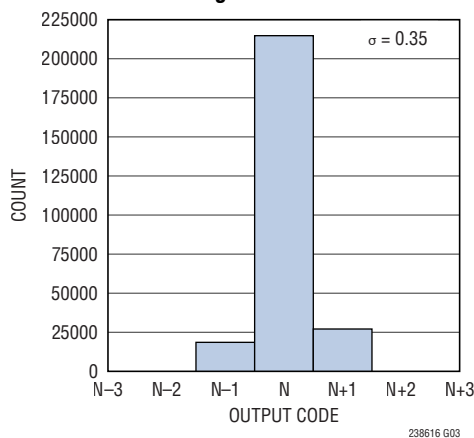
DC Histogram
