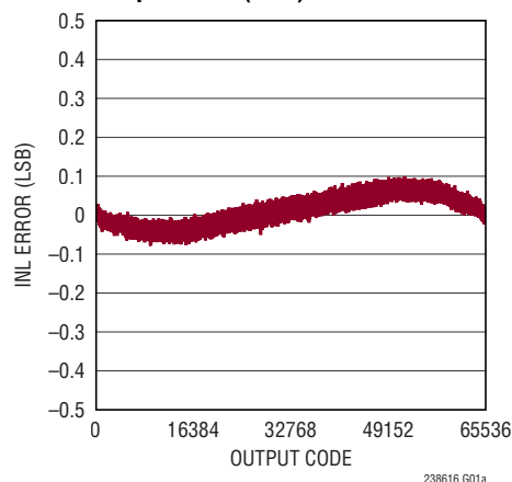
Integral Nonlinearity vs Output Code (LSB)
