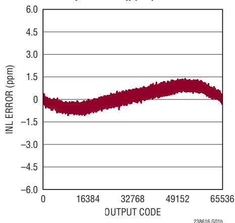
Integral Nonlinearity vs Output Code (ppm)
