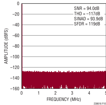
Figure 10. 32k Point FFT of the LTC2386-16, f_{\text{SMPL}} = 10\text{Msps} , f_{\text{IN}} = 2\text{kHz}
