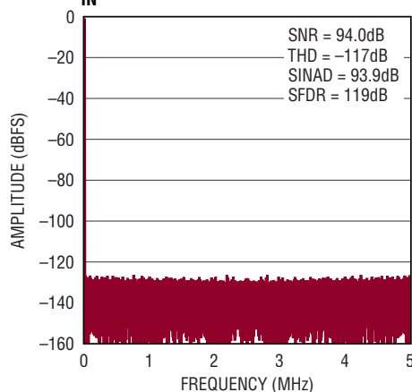
32k Point FFT f_{\text{SAMPL}} = 10\text{Mps} , f_{\text{IN}} = 2\text{kHz}
