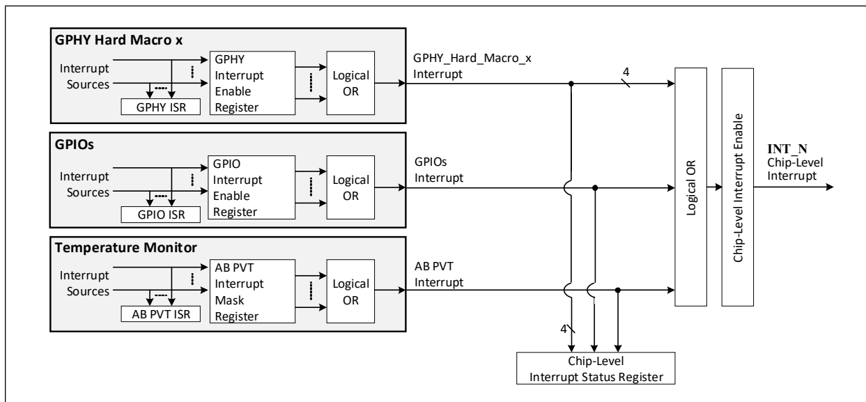
FIGURE 5-8: INTERRUPT STRUCTURE
