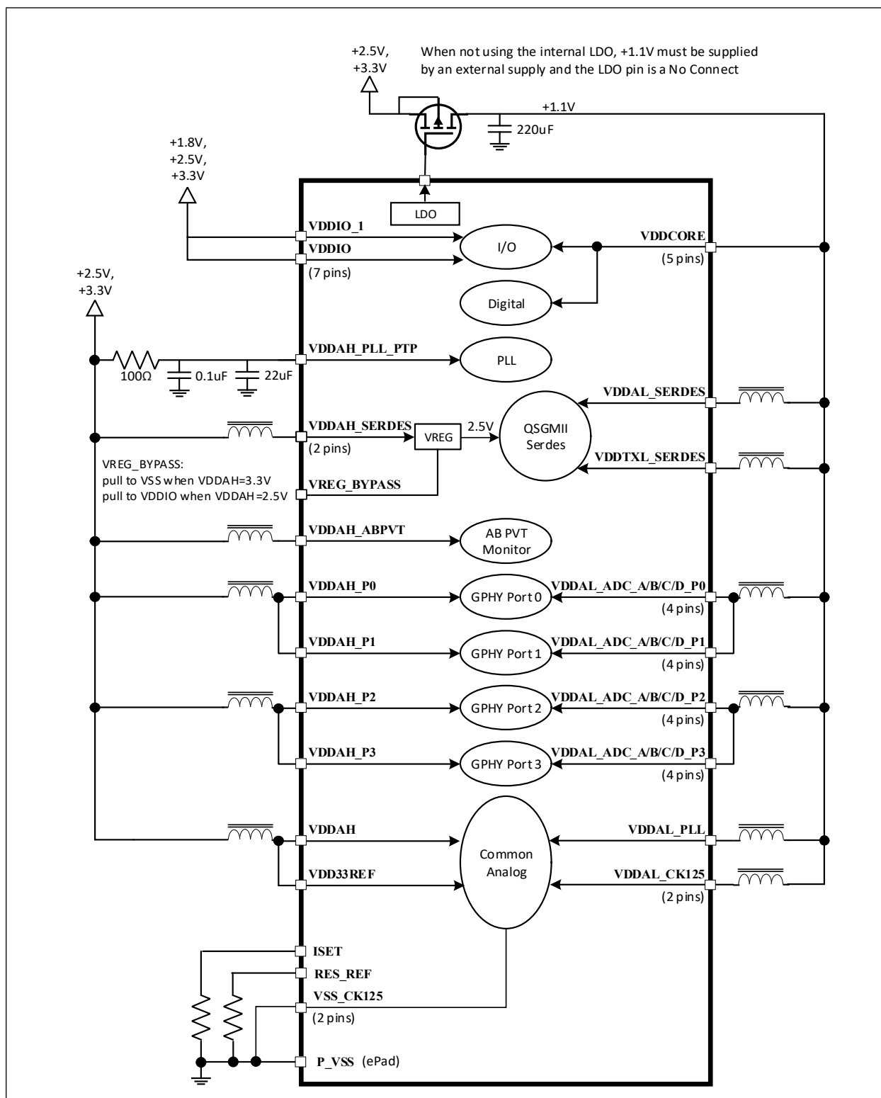
FIGURE 4-1: POWER CONNECTIONS
