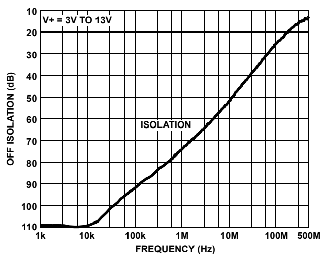
FIGURE 17. OFF ISOLATION
