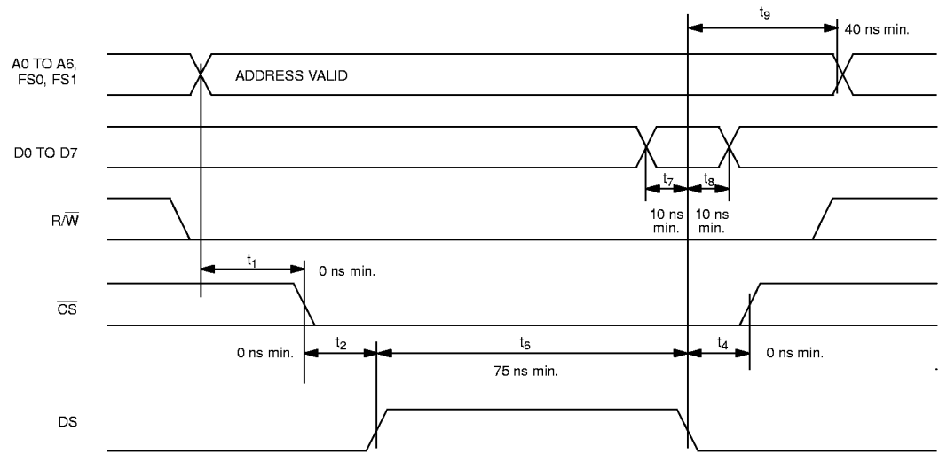
MOTOROLA BUS WRITE AC TIMING (BTS=1/MUX=0) Figure 13–13
