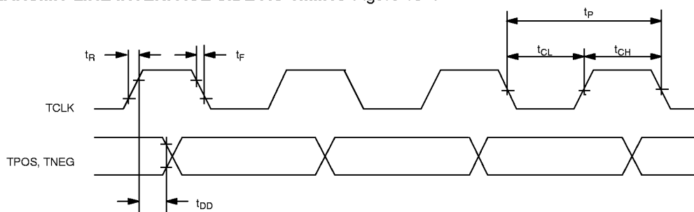
TRANSMIT LINE INTERFACE SIDE AC TIMING Figure 13-7
