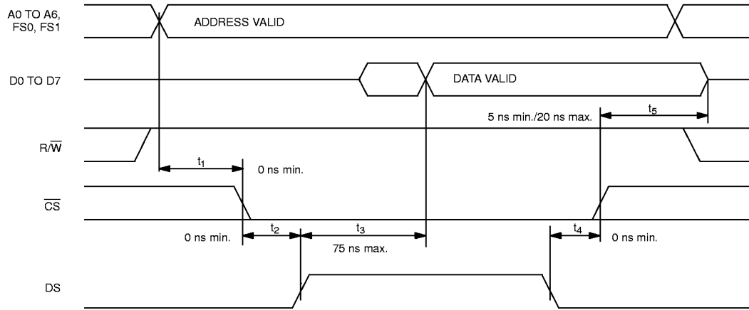
MOTOROLA BUS READ AC TIMING (BTS=1/MUX=0) Figure 13–12
