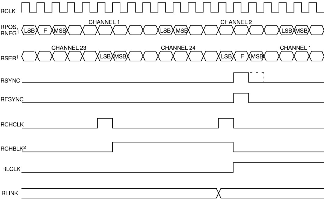
RECEIVE SIDE BOUNDARY TIMING (WITH ELASTIC STORE DISABLED) Figure 12–3
