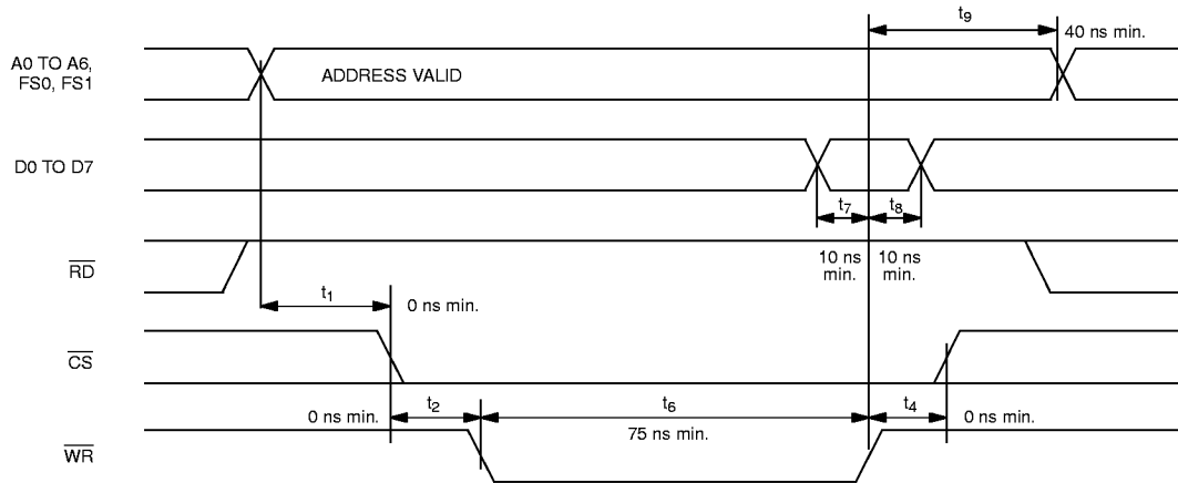
INTEL BUS WRITE AC TIMING (BTS=0/MUX=0) Figure 13–11
