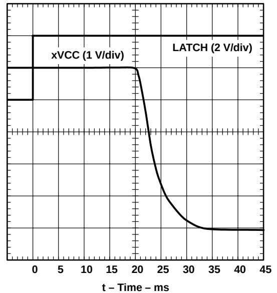
Figure 10. xVCC Propagation Delay and Fall Times With 100-μF Load, 5-V Switch
