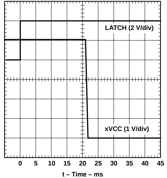
Figure 8. xVCC Propagation Delay and Fall Times With 1-μF Load, 5-V Switch
