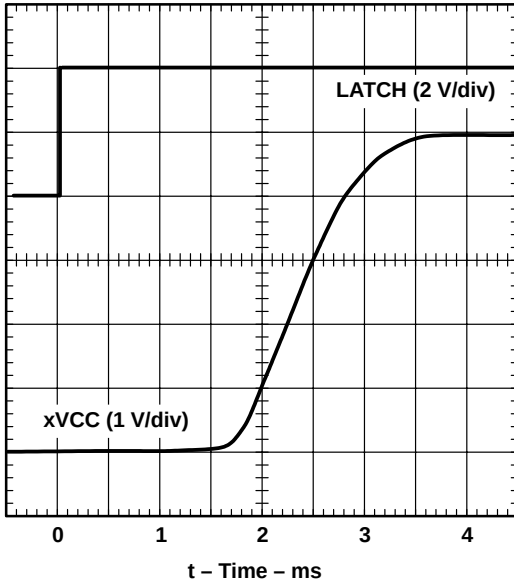
Figure 7. xVCC Propagation Delay and Rise Times With 1-μF Load, 5-V Switch
