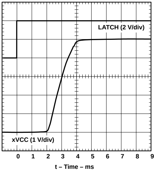
Figure 9. xVCC Propagation Delay and Rise Times With 100-μF Load, 5-V Switch
