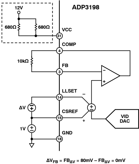
Figure 4. Positioning Voltage
