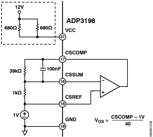
Figure 3. Current Sense Amplifier V_{Os}
