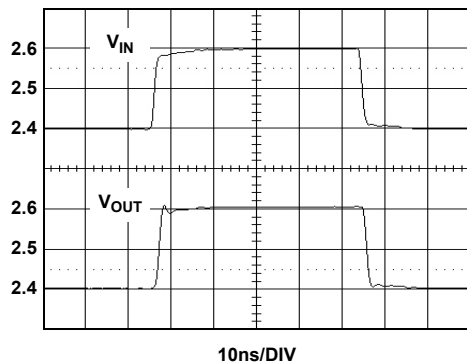
FIGURE 23. SMALL SIGNAL TRANSIENT RESPONSE
