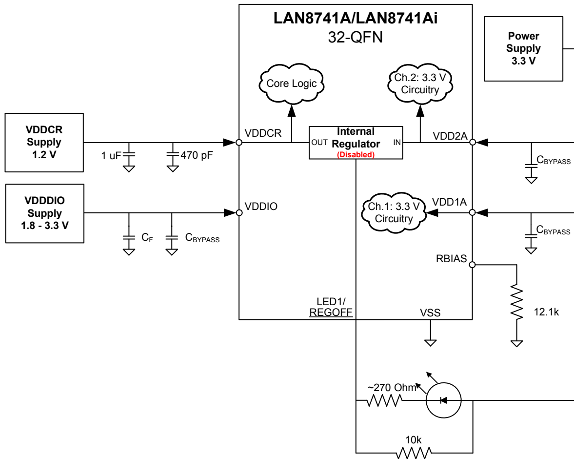
Figure 3.14 Power Supply Diagram (1.2 V Supplied by External Source)
