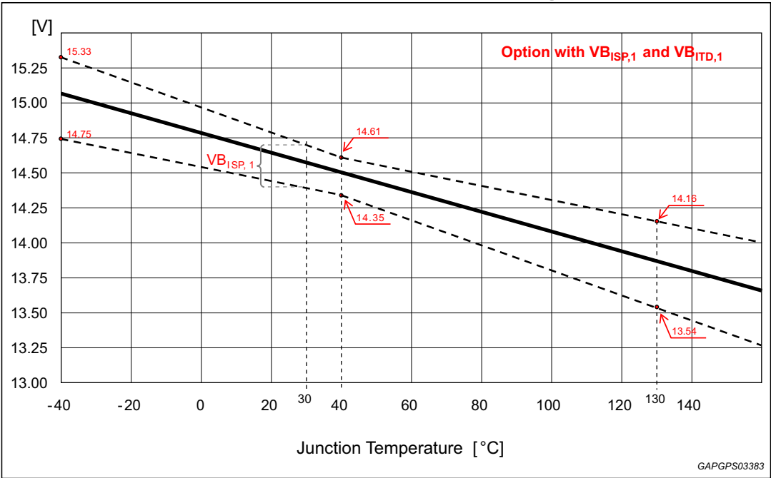
Figure 3. Internal regulation curves versus temperature @ F duty cycle = 15%
