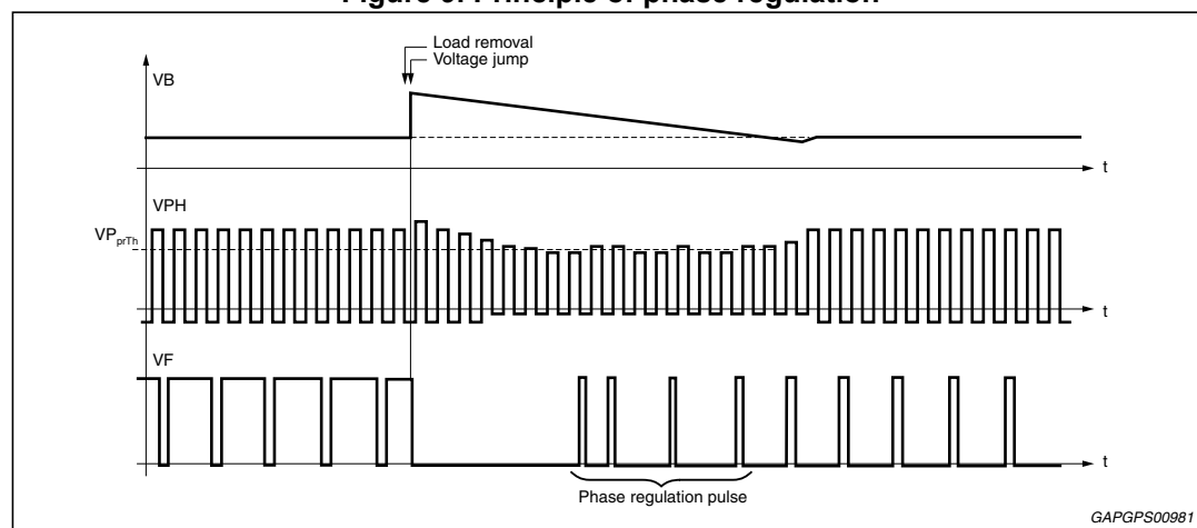
Figure 9. Principle of phase regulation
