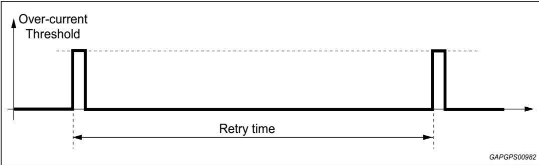
Figure 10. Retry time in case of over-current diagram
