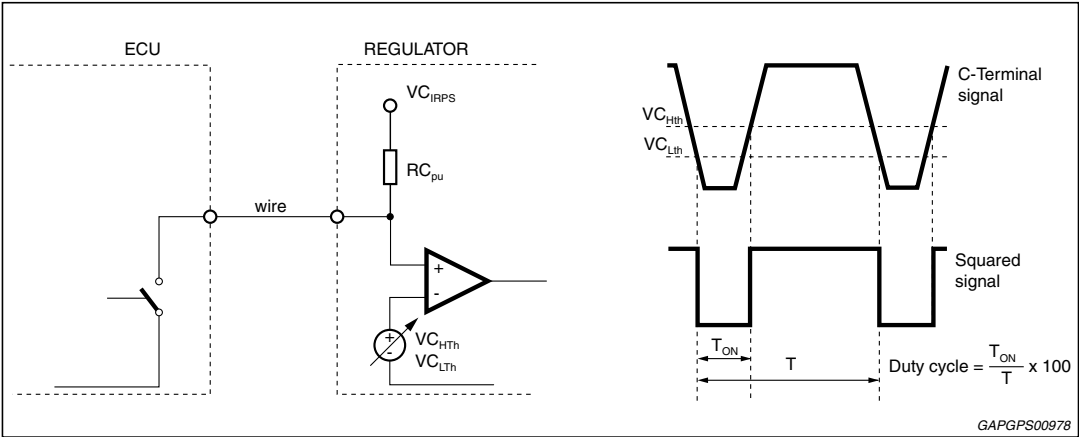
Figure 6. Pin 'C' circuit and waveform
