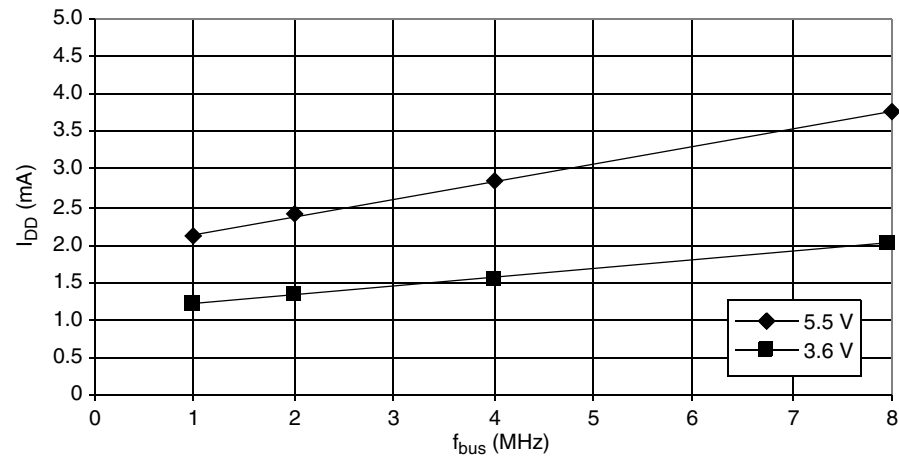
Figure 23-14. Typical Wait Mode I DD , with all Modules Disabled (–40 °C to 125 °C)
