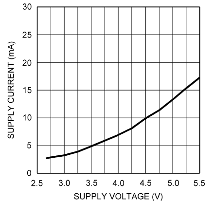
Supply Current vs Supply Voltage R_L = 8\Omega + 33\mu H
