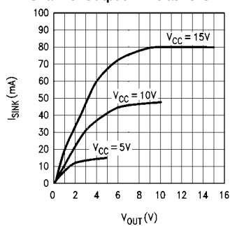
N-Channel Output Drive at 25^\circ\text{C}
