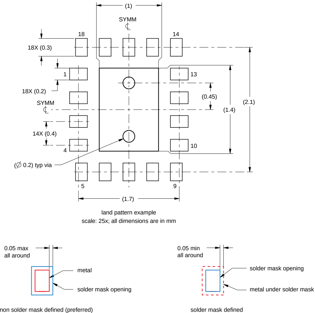
Fig 14. PCB footprint for SOT1442-1 (DHX2QFN18); reflow soldering
