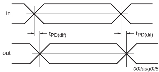
Fig 3. Propagation delay
