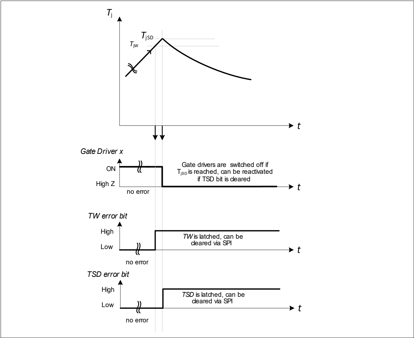
Figure 36 Overtemperature behavior
