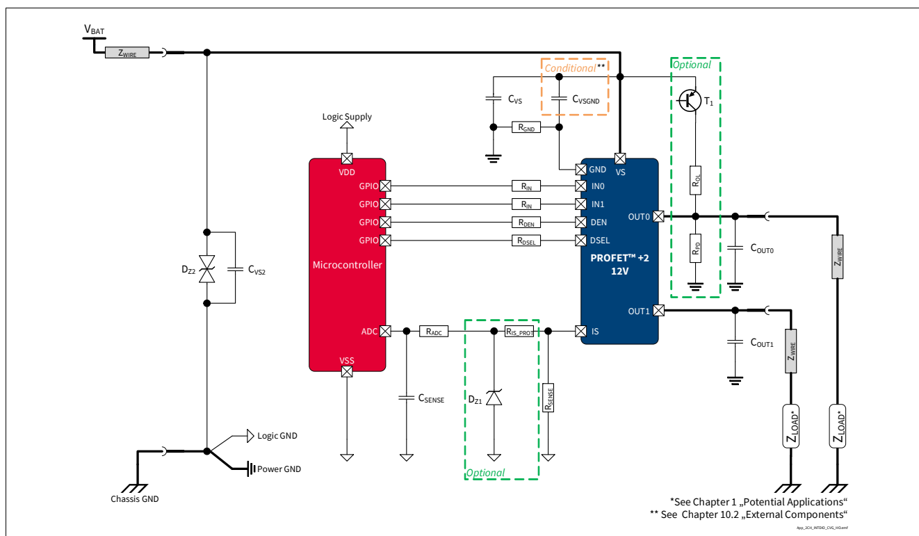
Figure 1 BTS7120-2EPA Application Diagram. Further information in Chapter 10
