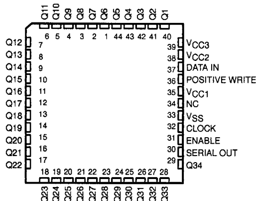
SN55563A ... FJ PACKAGE (TOP VIEW)
