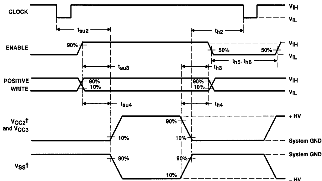
Figure 2. Control Input Timing Voltage Waveforms
