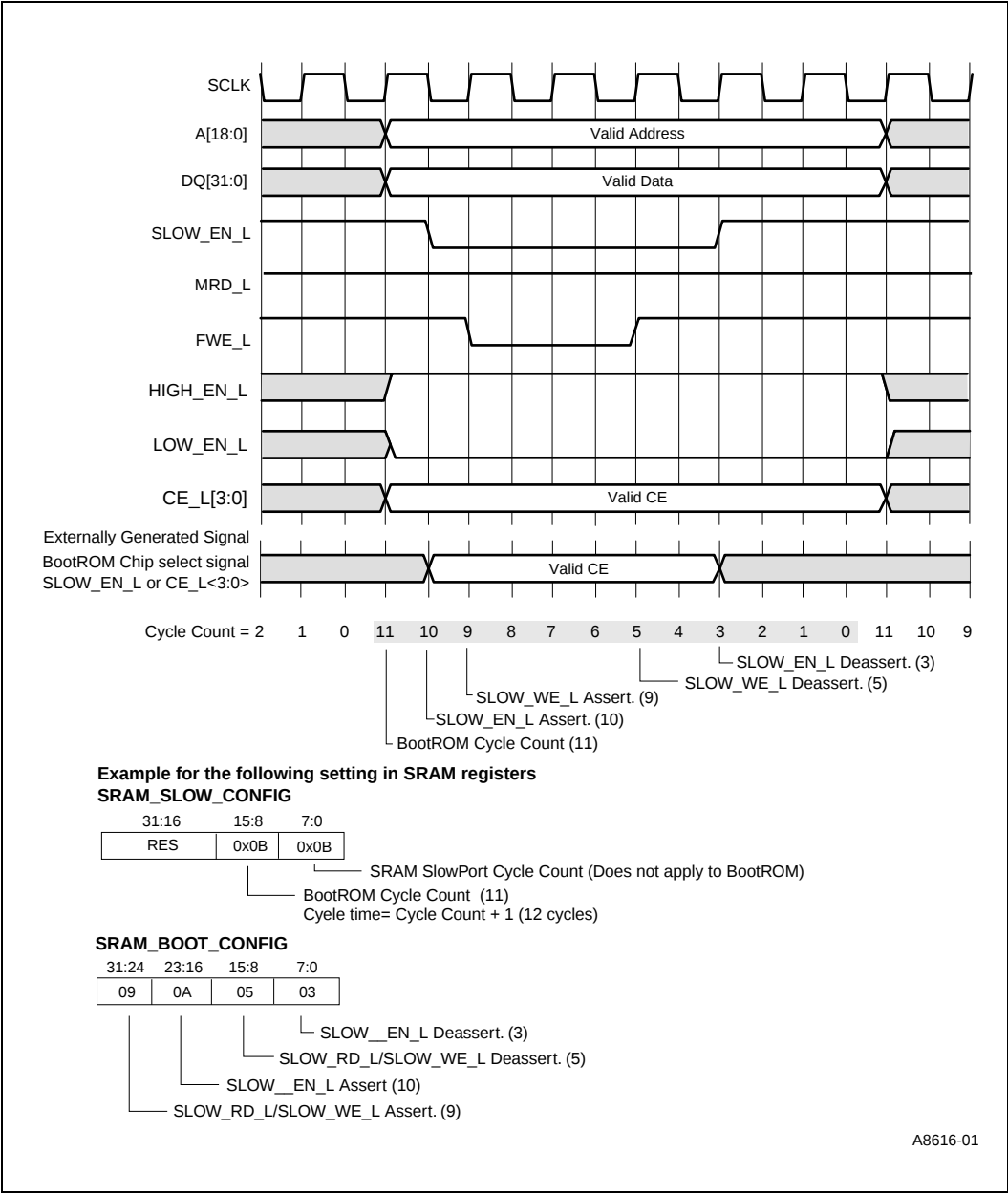
Figure 69. BootROM Write
