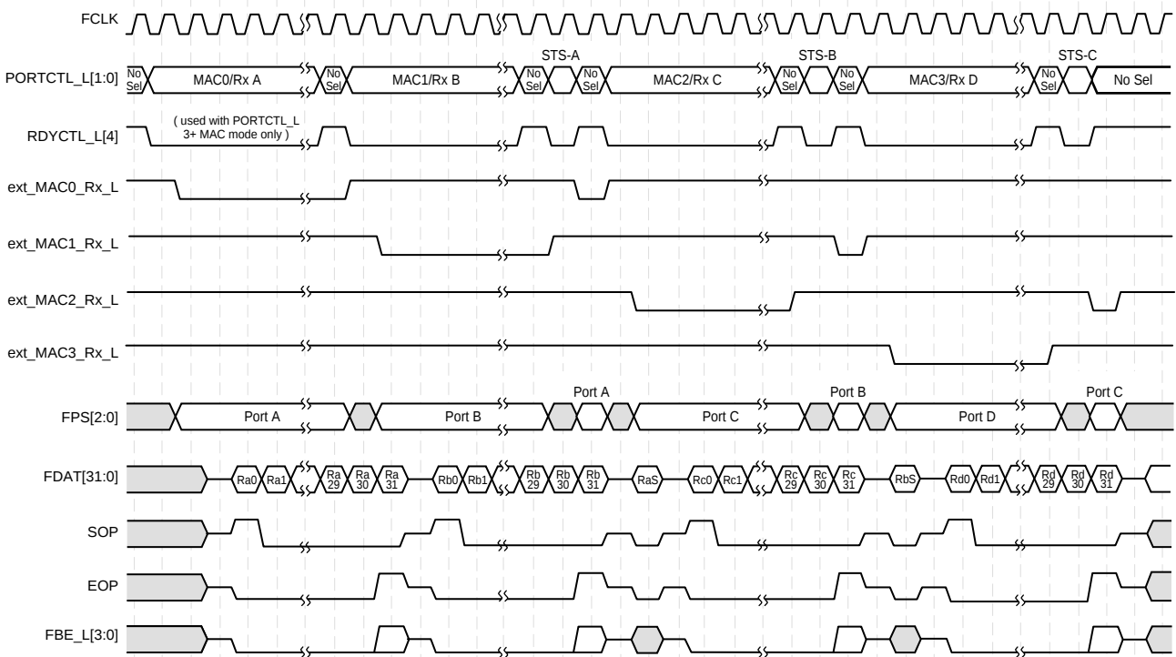
Figure 44. 32-Bit Unidirectional IX Bus Timing - Consecutive Receives, Two Element Transfers with 32-Bit Status
