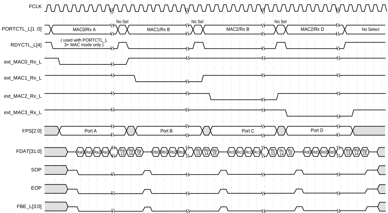
Figure 38. 32-Bit Unidirectional IX Bus Timing - Consecutive Receives, No EOP
