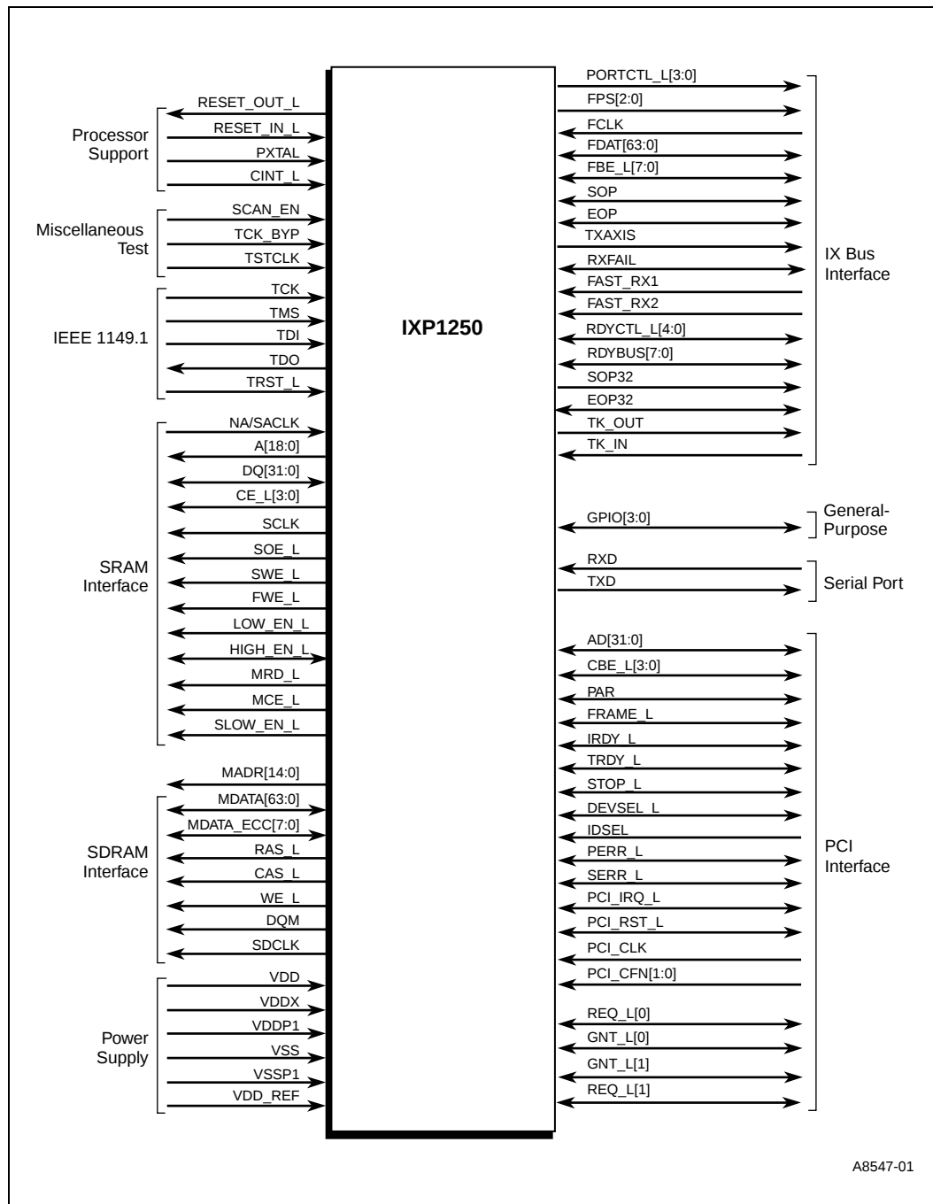
Figure 6. Pinout Diagram
