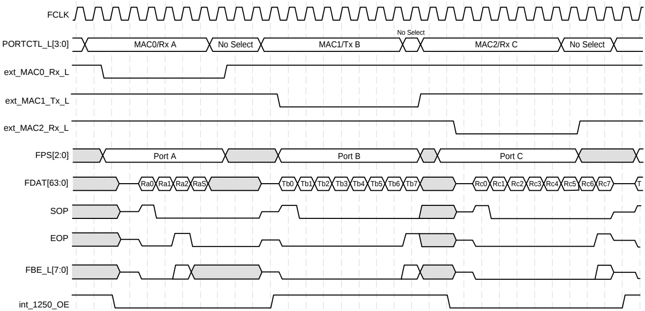
Figure 28. 64-Bit Bidirectional IX Bus Timing - Consecutive Receive and Transmit, EOP on 1st through 3rd Data Return with Status (3rd Data Return Shown)
