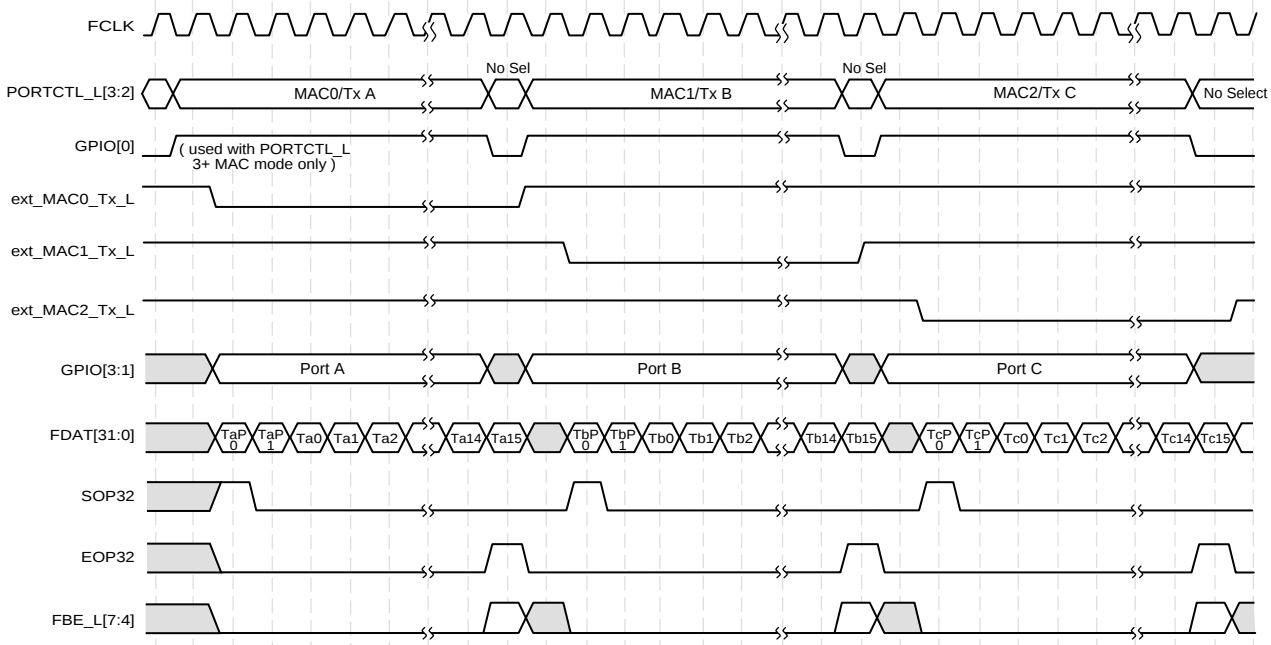
Figure 46. 32-Bit Unidirectional IX Bus Timing - Consecutive Transmits with Prepend, EOP
