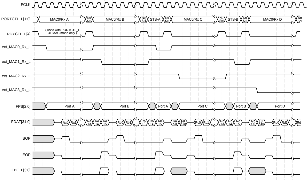
Figure 43. 32-Bit Unidirectional IX Bus Timing - Consecutive Receives, EOP, 64-Bit Status
