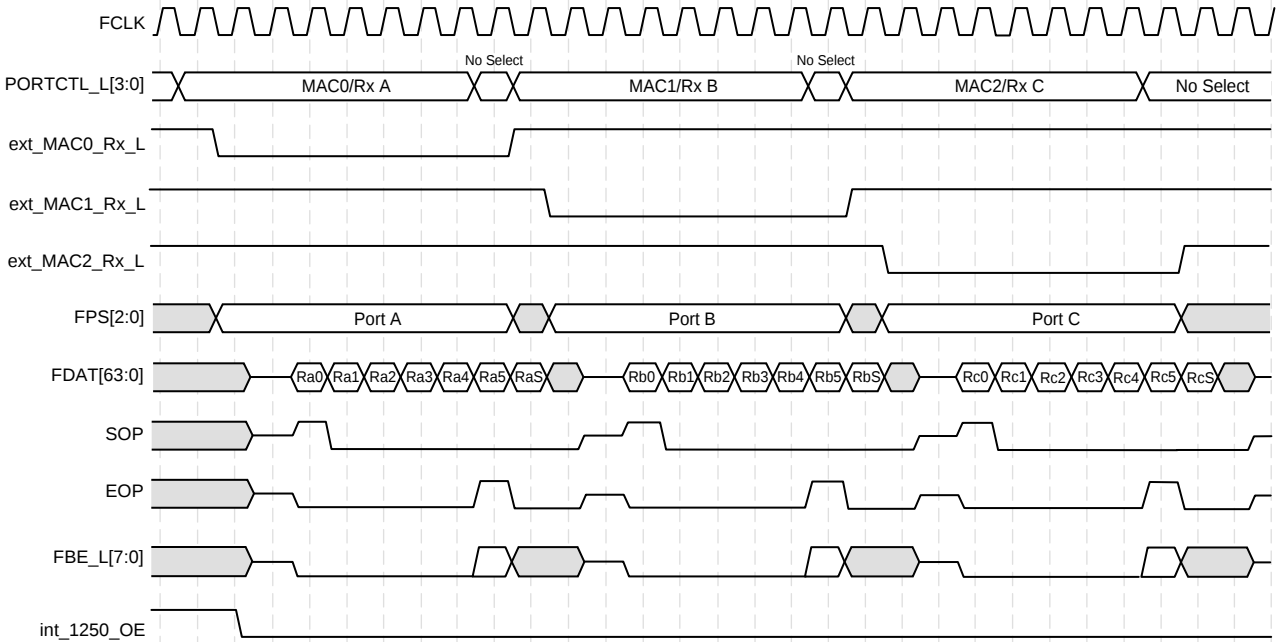
Figure 33. 64-Bit Bidirectional IXP Bus Timing - Consecutive Receives, EOP on 6th Data Return with Status
