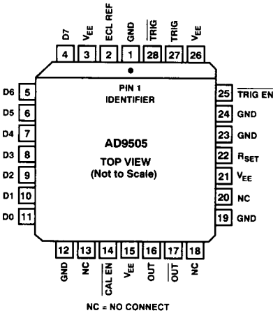
28-Lead PLCC
