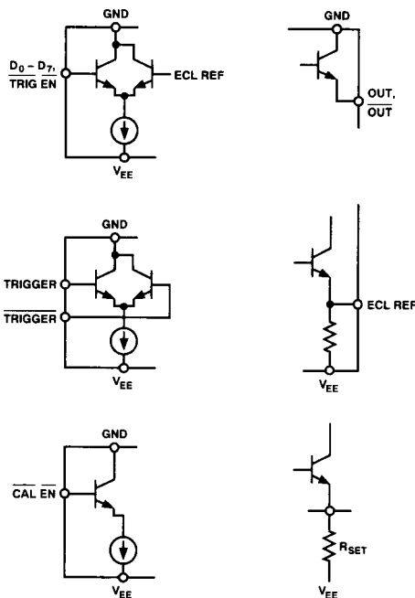
Equivalent Circuits
