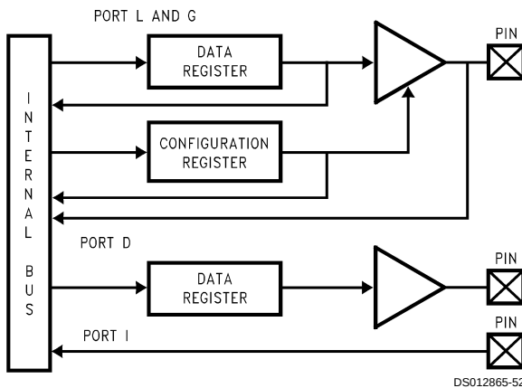
FIGURE 5. I/O Port Configurations
