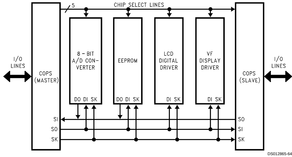
FIGURE 18. MICROWIRE/PLUS Application
