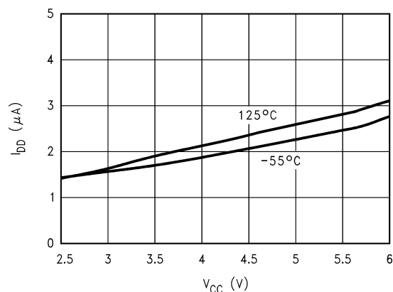
Halt — I_{DD} vs V_{CC} (COP8ACC5 Only)
