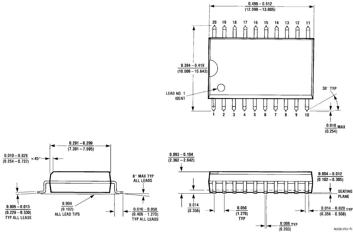
Order Number COP8ACC520M9 or COP8ACC520M8 NS Molded Package Number M20B
