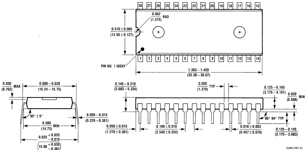
Order Number COP8ACC728N9-XE or COP8ACC728N8-XE NS Molded Package Number N28A
