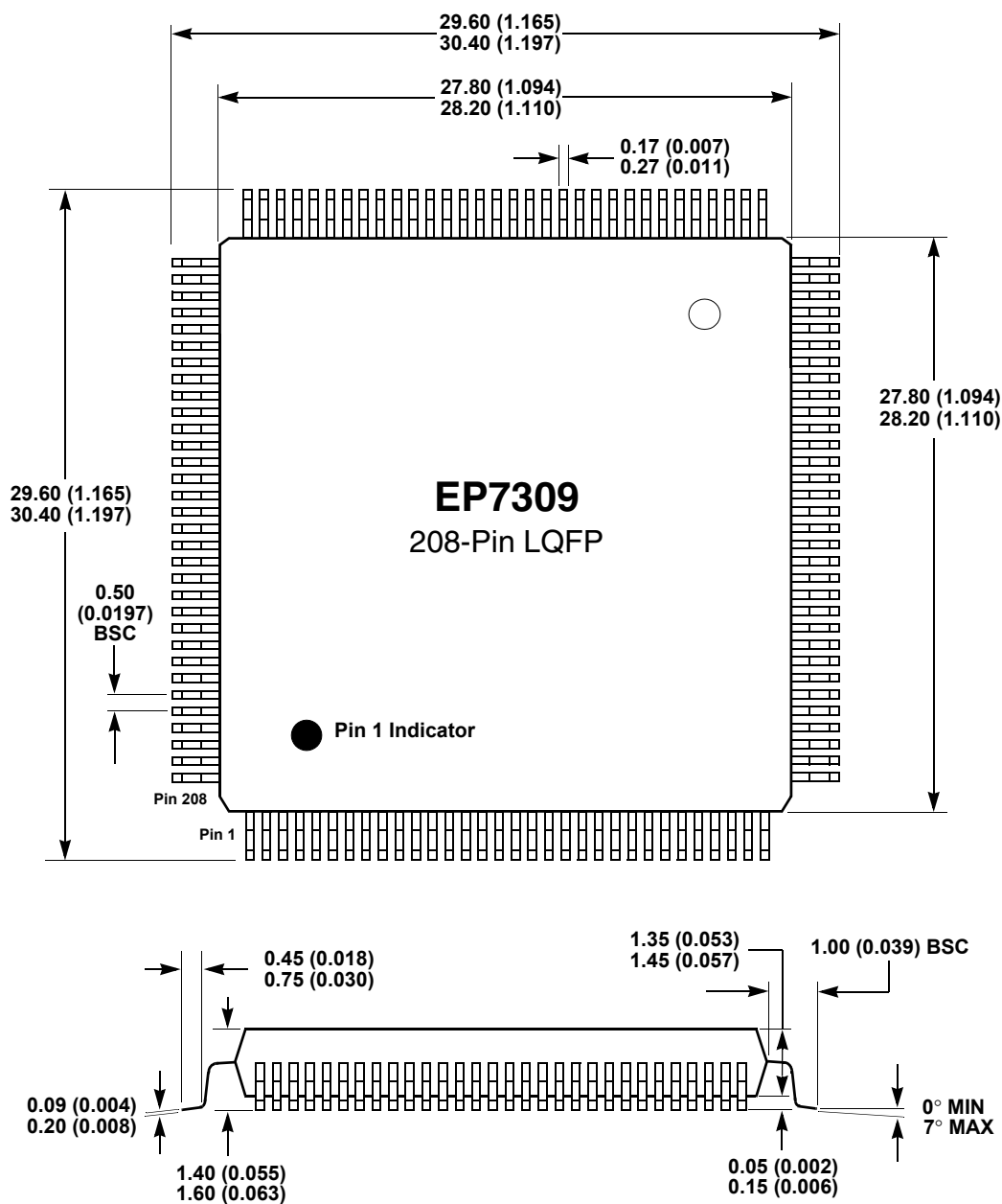
Figure 11. 208-Pin LQFP Package Outline Drawing
