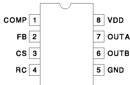
DIL-8, SOIC-8 (Top View) J or N Package, D Package
