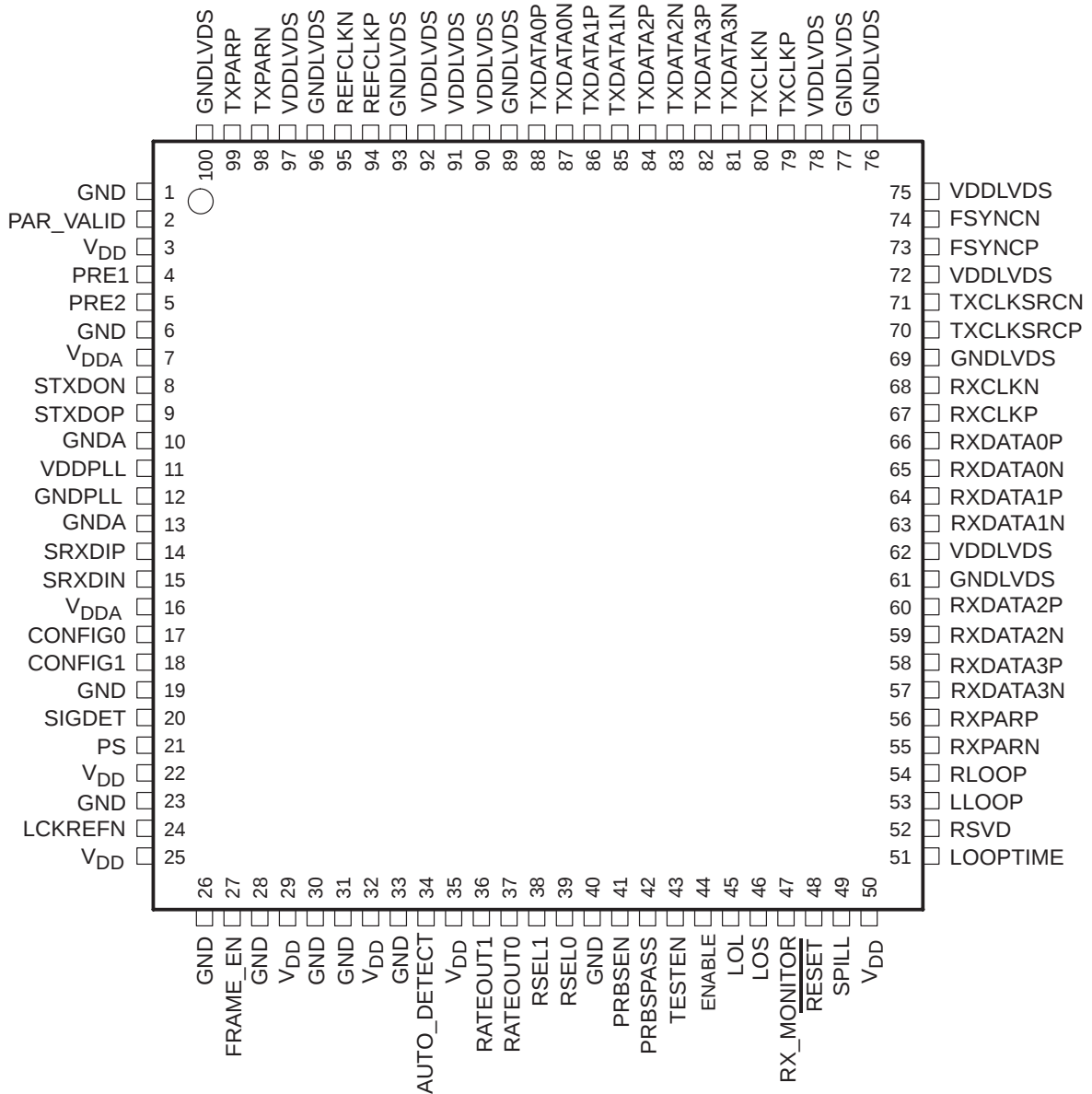
P2P PACKAGE (TOP VIEW)
