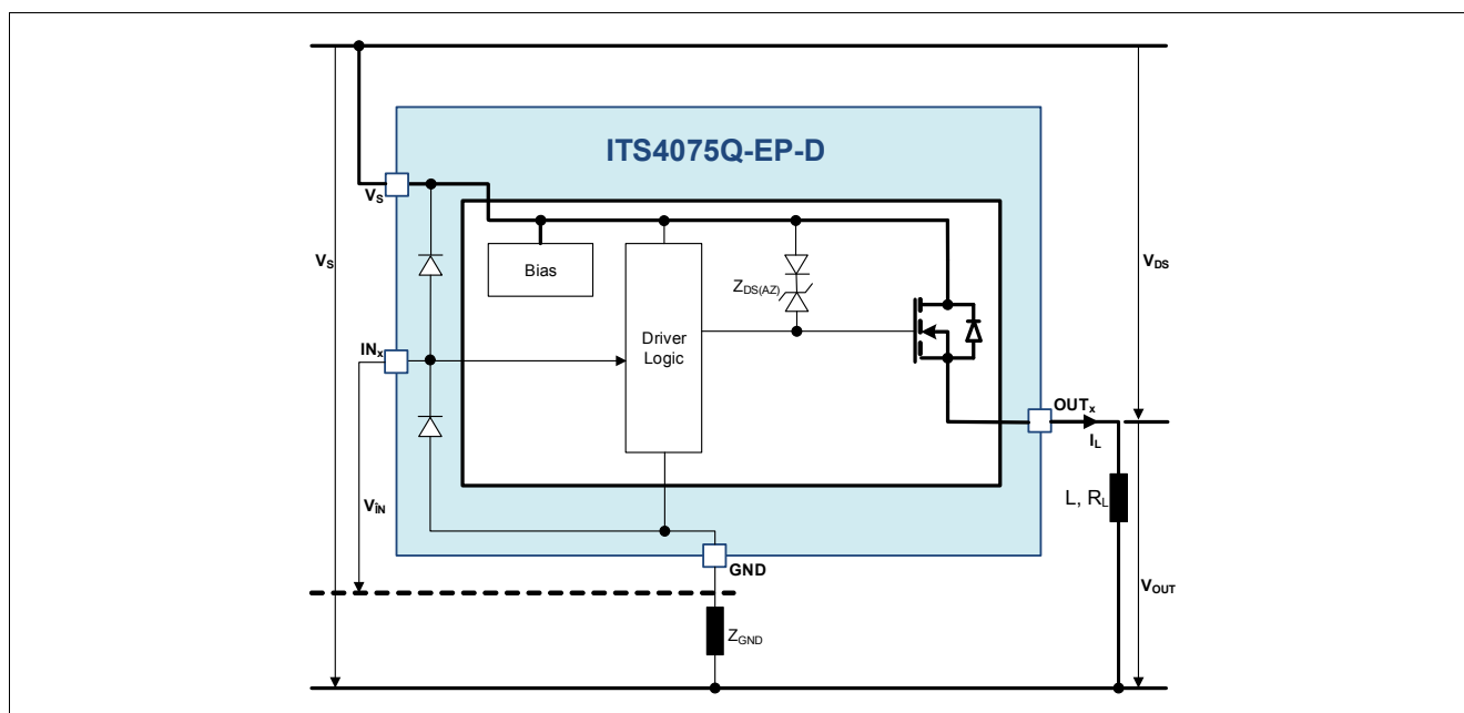
Figure 8 Output Clamp
