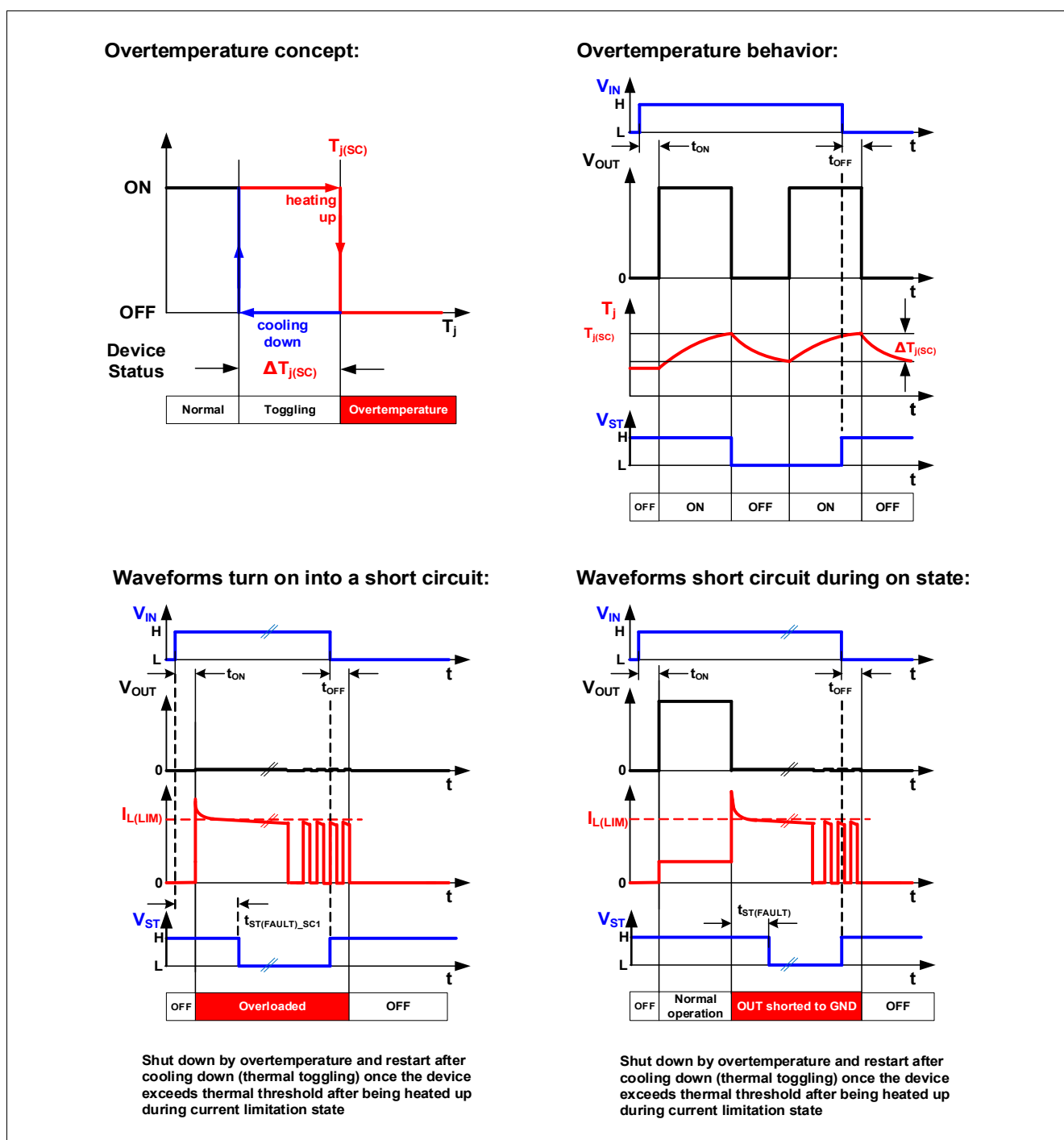
Figure 18 Protection behavior of the ITS4075Q-EP-D
