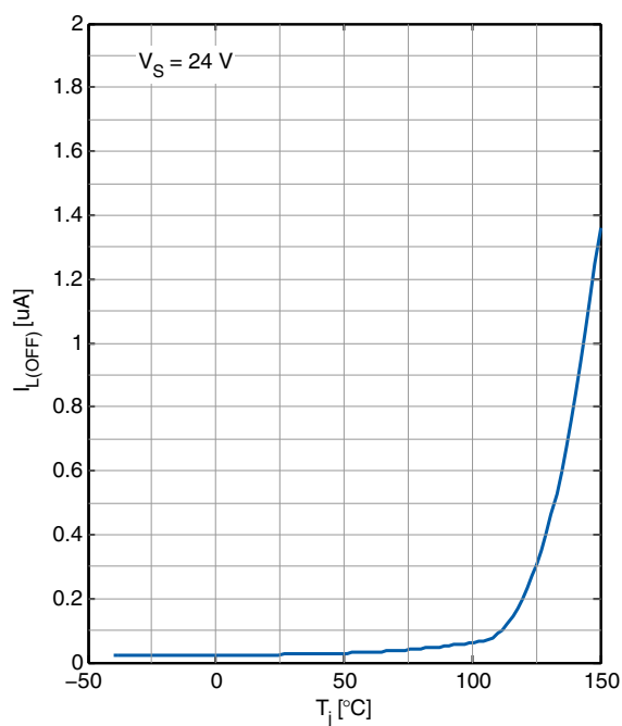
Leakage Current per channel I_{\text{L(OFF)}} versus Junction Temperature T_j
