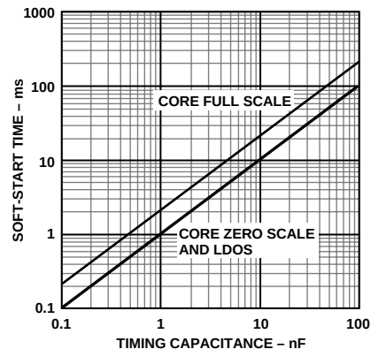
Figure 3. Soft-Start Time vs. Timing Capacitance
