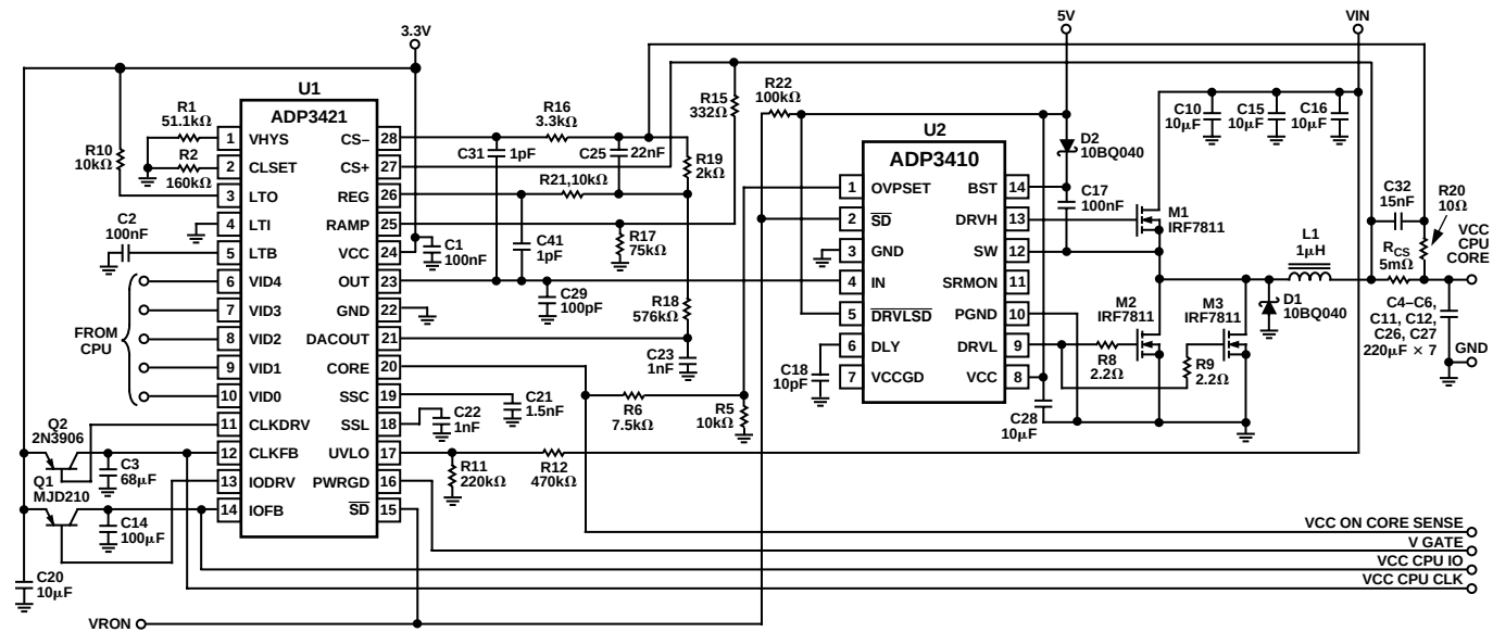
Figure 10. Mobile VRM Schematic
