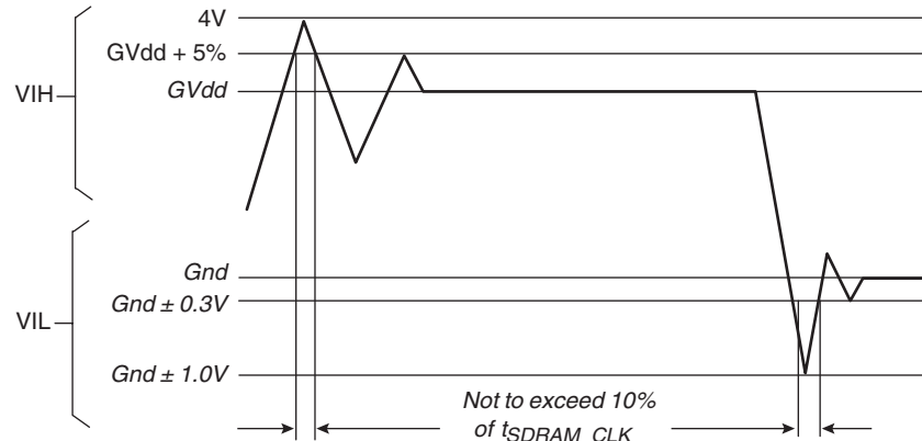
Figure 3-2. Overshoot/Undershoot Voltage
