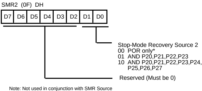
Figure 39. STOP-Mode Recovery Register 2 Write Only
