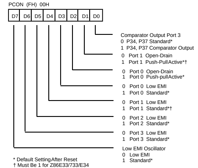
Figure 36. Port Configuration Register Write Only
