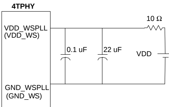
Figure 14. Pins 68-69 and 31-32 circuit diagram
