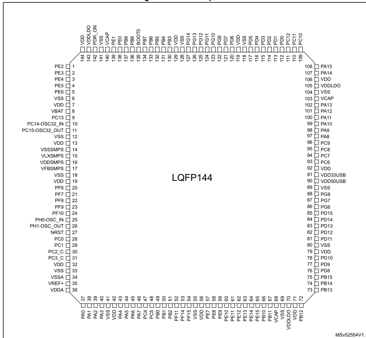
Figure 8. LQFP144 pinout
