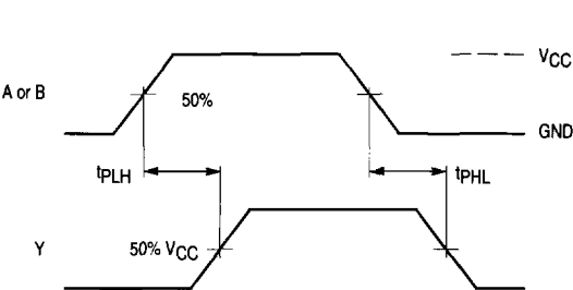
Figure 1. Switching Waveforms
