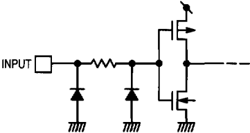
Figure 3. Input Equivalent Circuit
