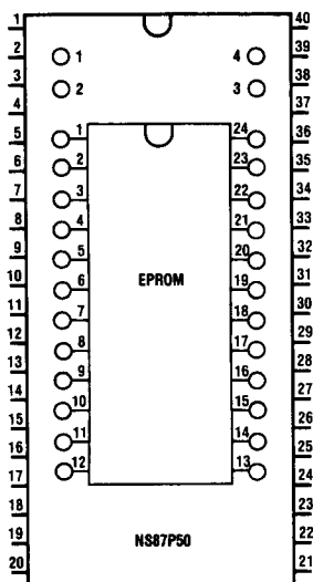
Pin Top View
