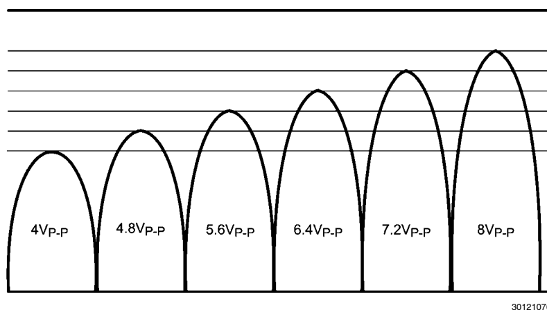
FIGURE 4. Voltage Limit Output Level
