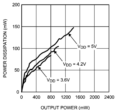
POWER DISSIPATION vs OUTPUT POWER R_L = 32\Omega , f = 1\text{kHz} Loudspeaker Mode 2
