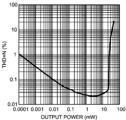
THD+N vs Output Power V_{DD} = 3.6V , HPV_{DD} = 1.8V , R_L = 32\Omega , f = 1kHz A_V = 6dB , Mode 4
