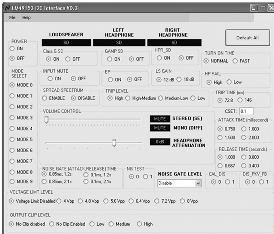
FIGURE 9. GUI Software
