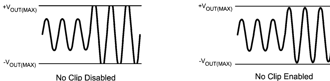
FIGURE 5. No Clip Function
