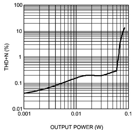
THD+N vs Output Power R_L = 32\Omega , f = 1kHz , Earpiece Mode
