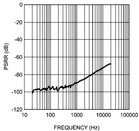
PSRR vs FREQUENCY V_{DD} = 3.6V , HPV_{DD} = 1.8V , V_{DD-RIPPLE} = 200mV_{P-P} R_L = 32\Omega , Mono Input, HP Mode
