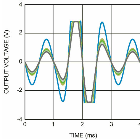
FIGURE 6. Clip Control Levels
