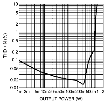
THD+N vs Output Power V_{DD} = 4.2V , R_L = 8\Omega , f = 1kHz A_V = 18dB , Mode 2
