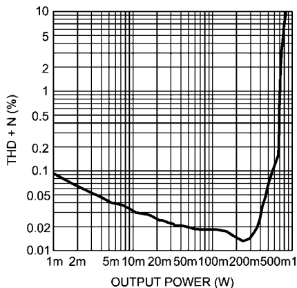
THD+N vs Output Power V_{DD} = 3.6V , R_L = 8\Omega , f = 1kHz A_V = 18dB , Mode 2
