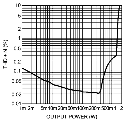
THD+N vs Output Power V_{DD} = 5.0V , R_L = 8\Omega , f = 1kHz A_V = 18dB , Mode 2
