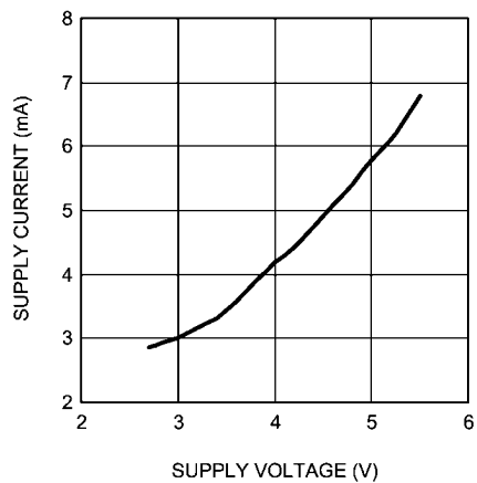
SUPPLY CURRENT vs SUPPLY VOLTAGE No Load, Loudspeaker Mode 2
