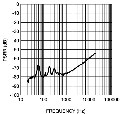
PSRR vs FREQUENCY V_{DD} = 3.6V , HPV_{DD} = 1.8V , V_{DD-RIPPLE} = 200mV_{P-P} R_L = 8\Omega , Mono Input, LS Mode
