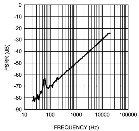
PSRR vs FREQUENCY V_{DD} = 3.6V , HPV_{DD} = 1.8V , V_{DD-RIPPLE} = 200mV_{P-P} R_L = 8\Omega , Stereo Input, LS Mode
