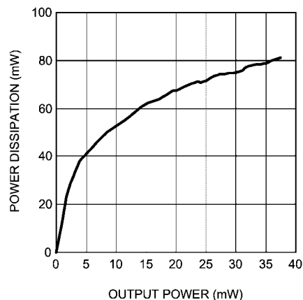
POWER DISSIPATION vs OUTPUT POWER V_{DD} = 3.6\text{V} , HPV_{DD} = 1.8\text{V} , R_L = 32\Omega , f = 1\text{kHz} Loudspeaker Mode 2
