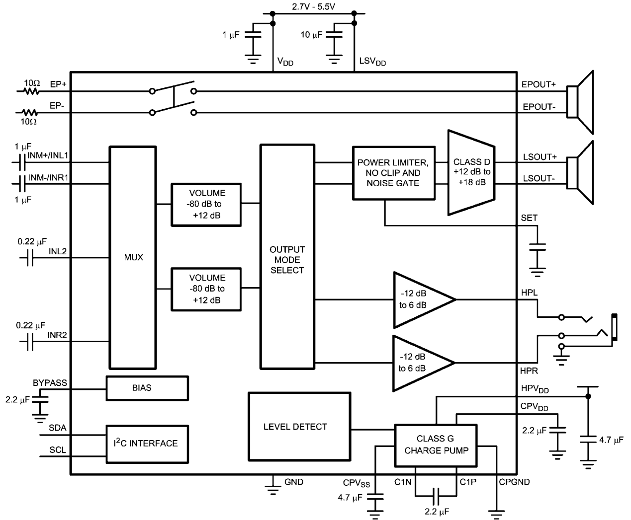
FIGURE 1. Typical Audio Amplifier Application Circuit
