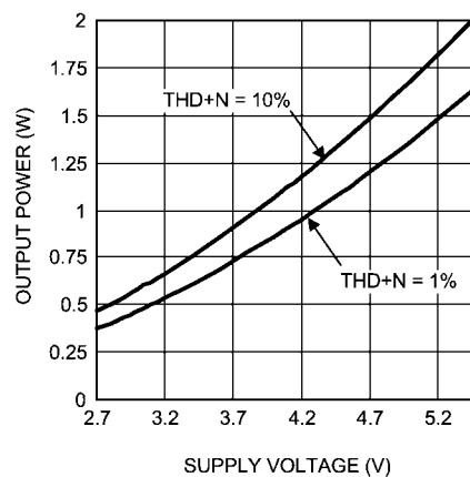
OUTPUT POWER vs SUPPLY VOLTAGE R_L = 8\Omega , f = 1\text{kHz}
