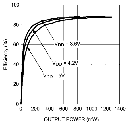
EFFICIENCY vs OUTPUT POWER R_L = 8\Omega , f = 1\text{kHz} , Loudspeaker Mode 2
