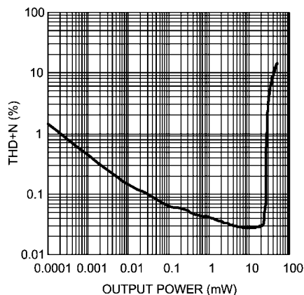
THD+N vs Output Power V_{DD} = 3.6V , HPV_{DD} = 1.8V , R_L = 16\Omega , f = 1kHz A_V = 6dB , Mode 4
