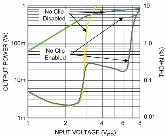
FIGURE 8. No Clip Function V_{DD} = 3.3V , R_L = 8\Omega + 30\mu H f_{IN} = 1kHz , LS\_GAIN = 0 Gray, Yellow = THD+N vs Input Voltage
