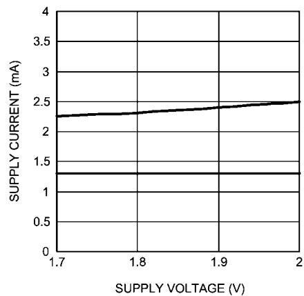
SUPPLY CURRENT vs SUPPLY VOLTAGE No Load, Loudspeaker Mode 4
