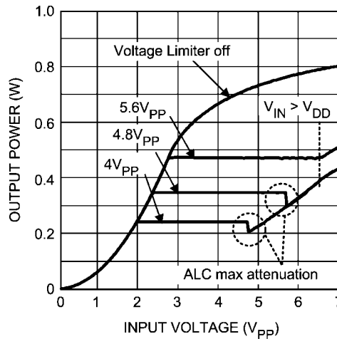
FIGURE 7. Voltage Limiter Function
