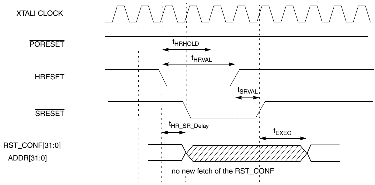
Figure 5. HRESET Behavior
