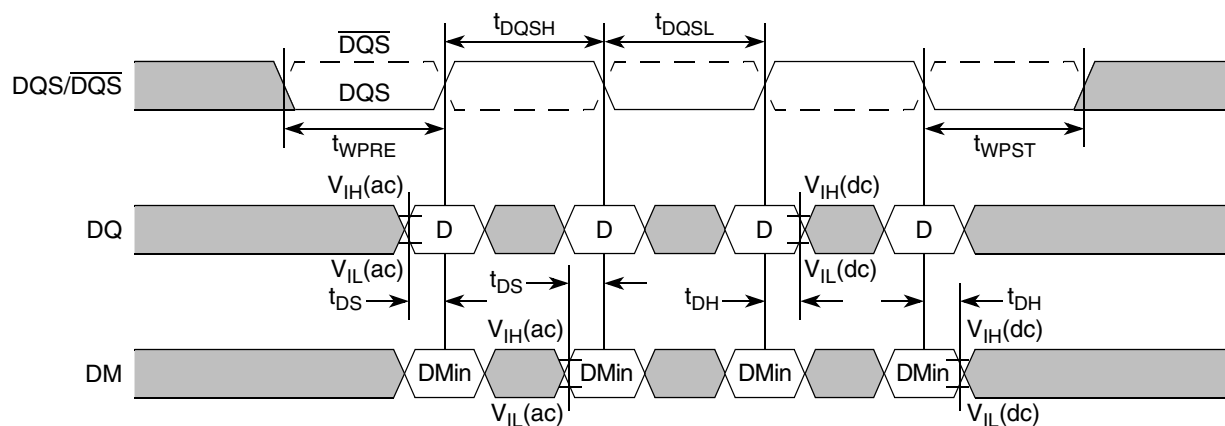
Figure 7. DDR Write Timing
