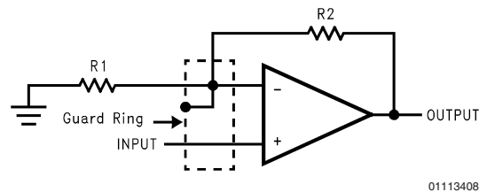
FIGURE 7. Guard Ring Connections Non-Inverting Amplifier
