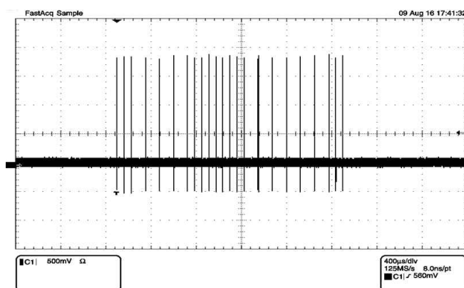
Figure 6-11. Auto-Negotiation FLP
