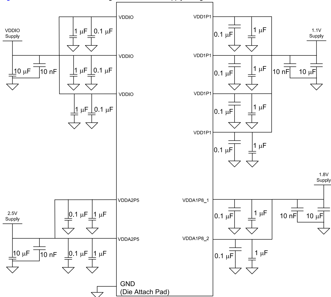
Figure 9-3. Three-Supply Configuration
