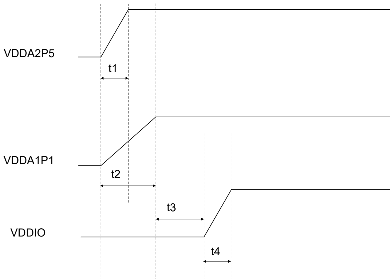
Figure 9-2. Two-Supply Sequence Diagram
