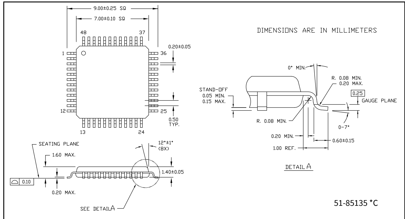
Figure 8 48-Pin 7 x 7 x 1.4-mm TQFP package (0.5-mm Pitch) outline
