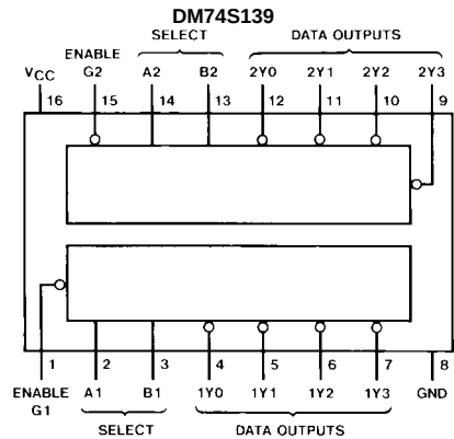
DM74S139
