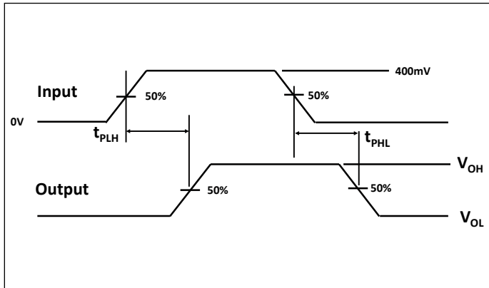
Figure 4. Propagation Delay
