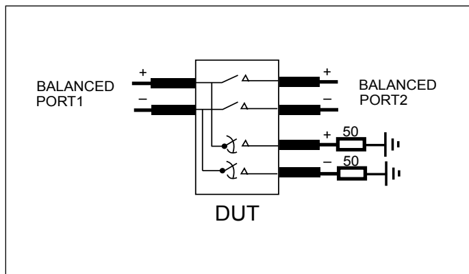
Figure 2. Off-isolation Setup
