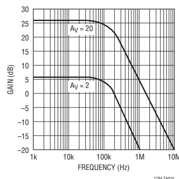
Programmable Gain Amplifier Frequency Response
