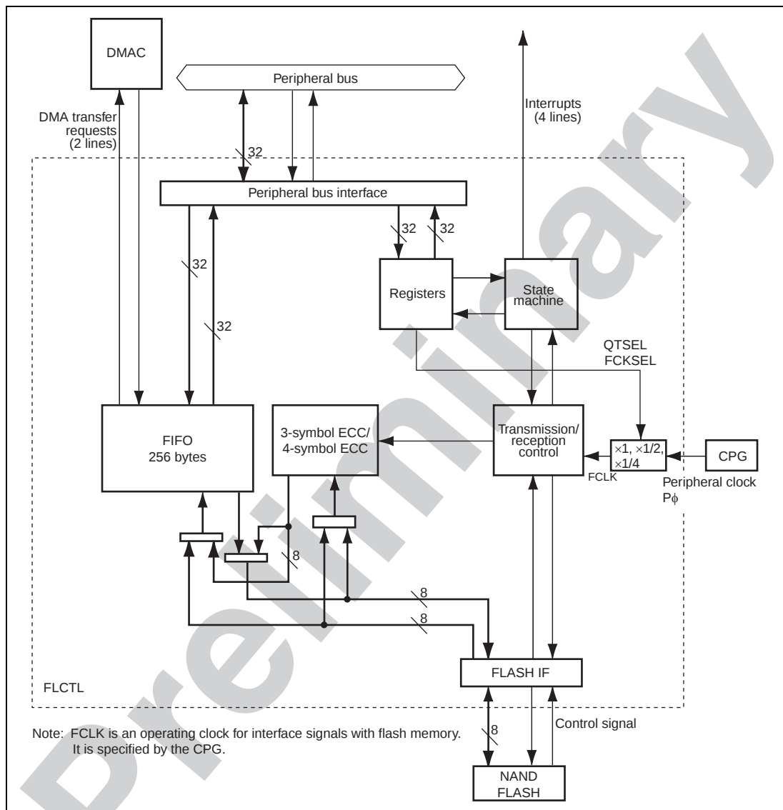
Figure 24.1 FLCTL Block Diagram
