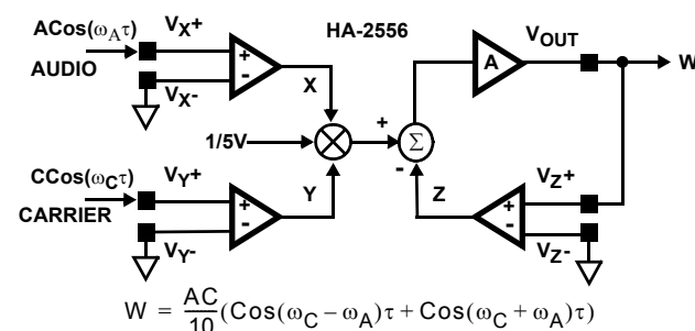
FIGURE 6. AM SIGNAL GENERATION
