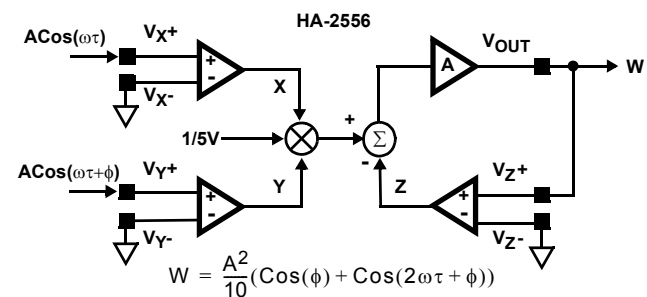
FIGURE 8. PHASE DETECTION
