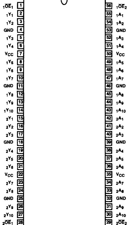
CD74LPT16827 (SSOP, TSSOP) TOP VIEW
