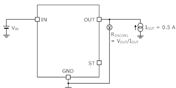
Measurement Circuit for Figure 6 and Figure 7
