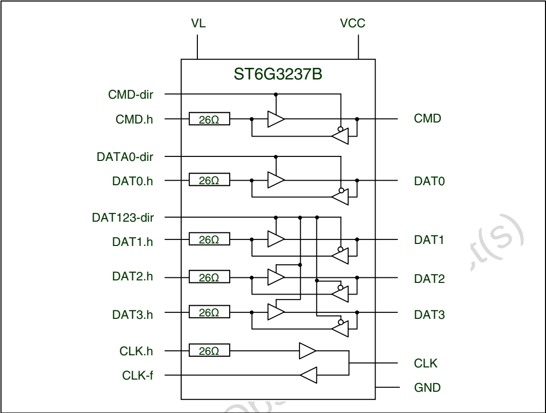
Figure 1. Logic diagram
