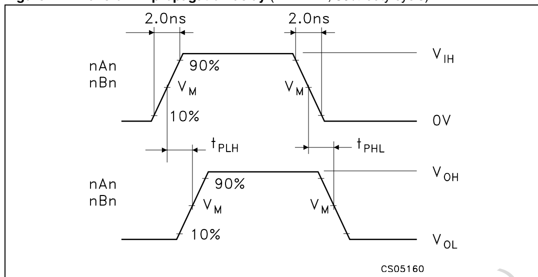
Figure 4. Waveform - propagation delay ( f = 1\text{MHz} , 50% duty cycle)
