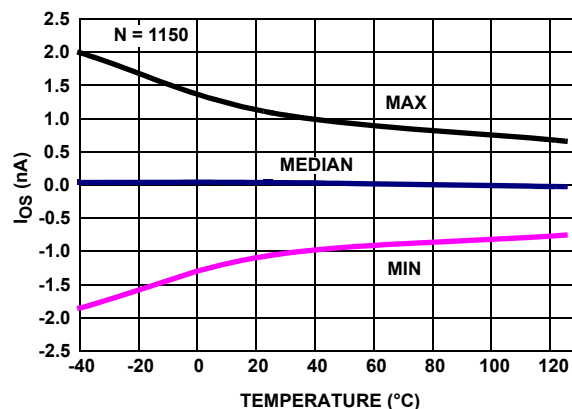
FIGURE 24. I_{OS} vs TEMPERATURE, V_+ , V_- = \pm 2.5V
