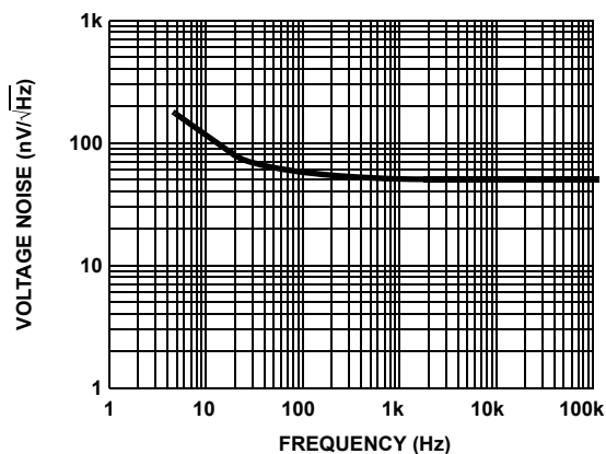
FIGURE 8. VOLTAGE NOISE vs FREQUENCY
