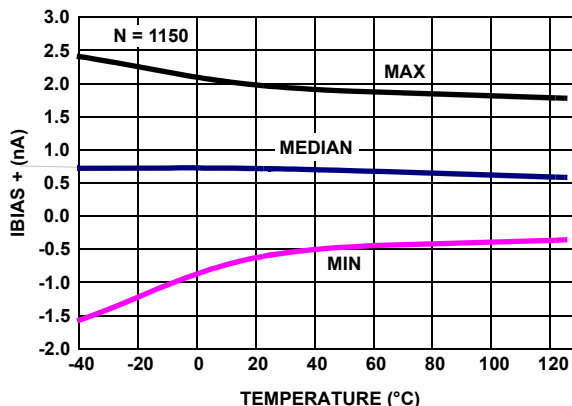
FIGURE 22. I_{BIAS+} vs TEMPERATURE, V_+ , V_- = \pm 1.2V
