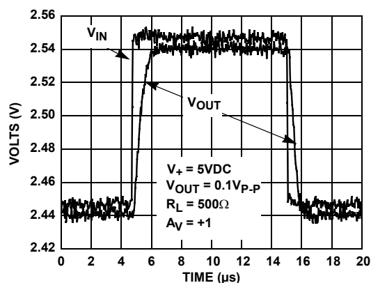
FIGURE 10. SMALL SIGNAL TRANSIENT RESPONSE
