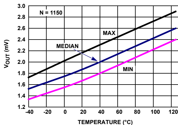
FIGURE 32. V_{OUT} LOW vs TEMPERATURE, V_+ , V_- = \pm 2.5V , R_L = 100k
