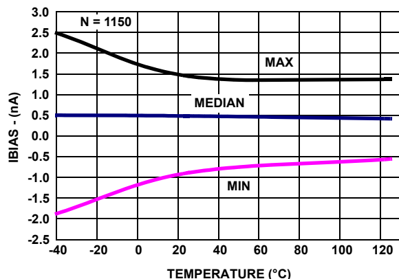
FIGURE 21. I_{BIAS-} vs TEMPERATURE, V_+ , V_- = \pm 2.5V
