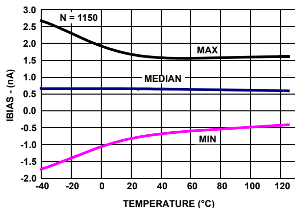
FIGURE 23. I_{BIAS-} vs TEMPERATURE, V_+ , V_- = \pm 1.2V
