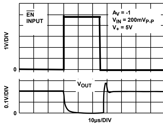
FIGURE 12. ENABLE TO OUTPUT DELAY TIME
