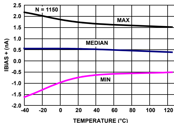
FIGURE 20. I_{BIAS+} vs TEMPERATURE, V_+ , V_- = \pm 2.5V
