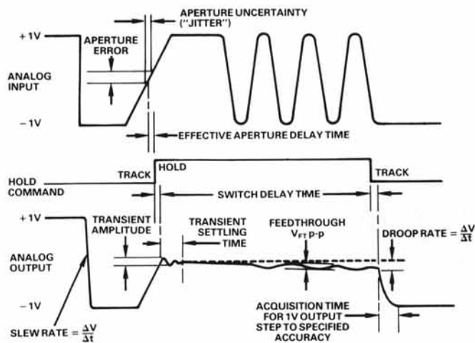
Figure 2. Track/Hold Waveforms
