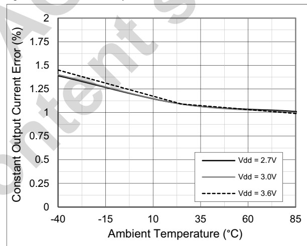
Figure 19. \Delta I_{COC} vs. Temperature; R_{EXT} = 10k\Omega
