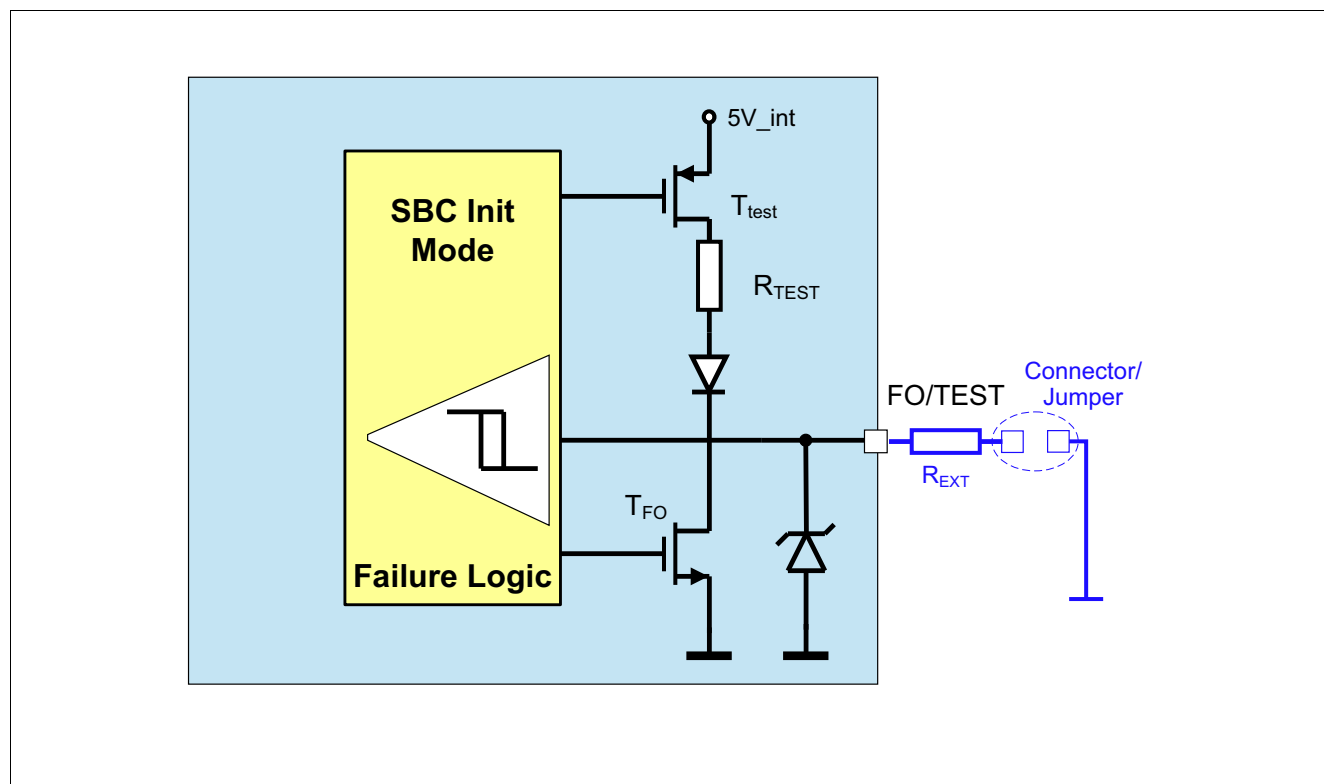
Figure 53 Hint for Increasing the Robustness of pin FO/TEST during Debugging or Programming
