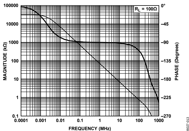
Figure 9. Open-Loop Transimpedance Gain and Phase vs. Frequency
