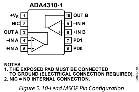
Figure 5. 10-Lead MSOP Pin Configuration
