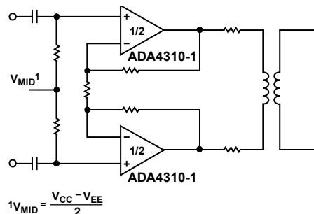
Figure 3. Typical PLC Driver Application
