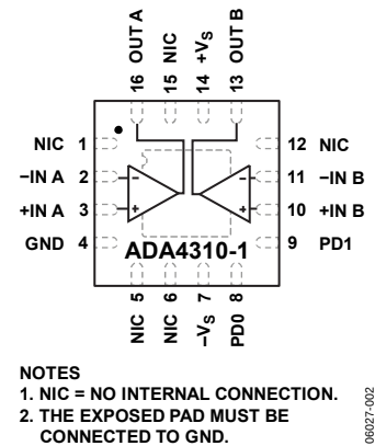
Figure 6. 16-Lead LFCSP Pin Configuration
