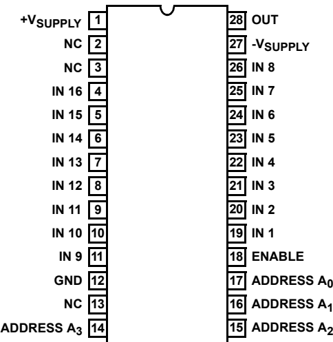
HI-506 (CERDIP, SOIC) TOP VIEW
