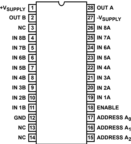
HI-507 (PDIP, CERDIP) TOP VIEW
